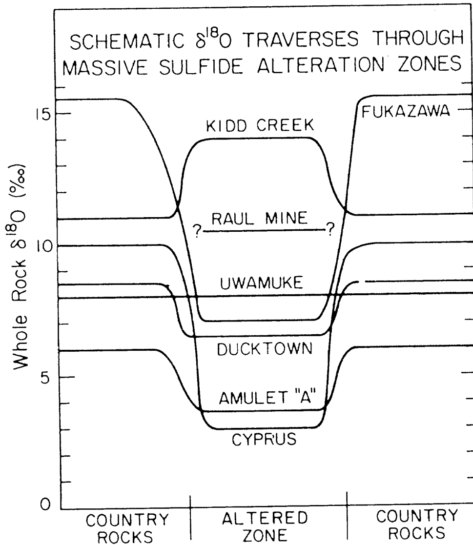
FIG. 75. Generalized distribution of oxygen isotope data across the footwall alteration zones of selected massive sulfide deposits. (After Beaty and Taylor, in prep., courtesy D. Beaty, Noranda Ltd., Denver.)
