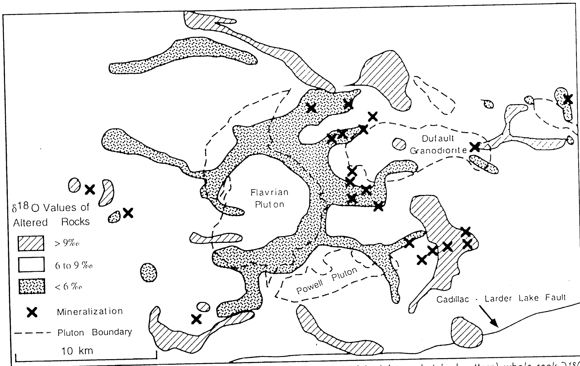
FIGURE 4. Distribution of ^{18}\text{O} depleted (stippled pattern) and ^{18}\text{O} enriched (cross-hatched pattern) whole rock \delta^{18}\text{O} values in the Noranda mining district, Quebec. X's indicate sites of volcanogenic massive sulfide mineralization. Note close correlation of low ^{18}\text{O} "fingers" and sites of mineralization (From Cathles, 1993).
