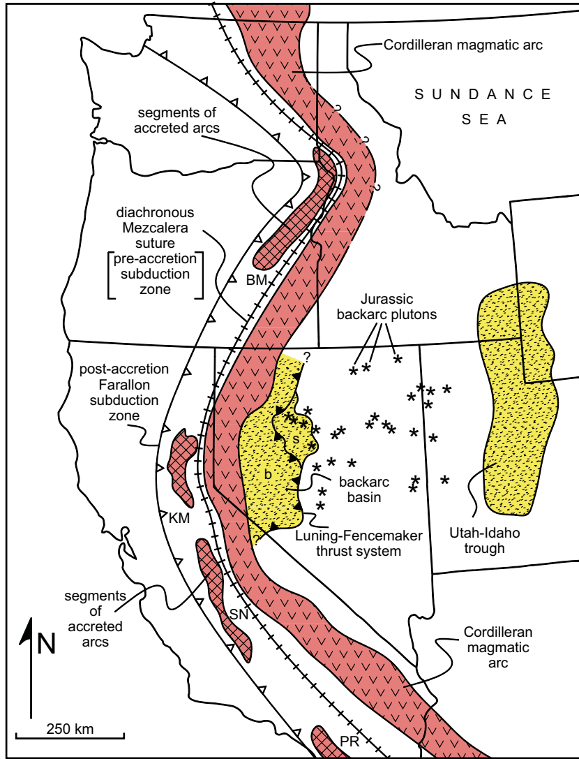
Figure 6. Triassic-Jurassic (post-Sonoma) paleotectonic map of the Great Basin and adjacent areas after mid–Early Triassic initiation of the Cordilleran magmatic arc. Positions of Cordilleran magmatic arc and accreted arc have been adjusted to compensate for younger Cretaceous-Paleogene displacements. Accreted intraoceanic arc segments are shown schematically for the Blue Mountains (BM), western Klamath Mountains (KM), Sierra Nevada foothills (SN), and Peninsular Ranges (PR). Shelfal (s) and basinal (b) facies are shown schematically within the backarc basin of western Nevada. Locations of backarc Jurassic plutons are after Elison et al. (1990) and Elison (1995) . Configuration of Utah-Idaho trough is after Peterson (1972) .
