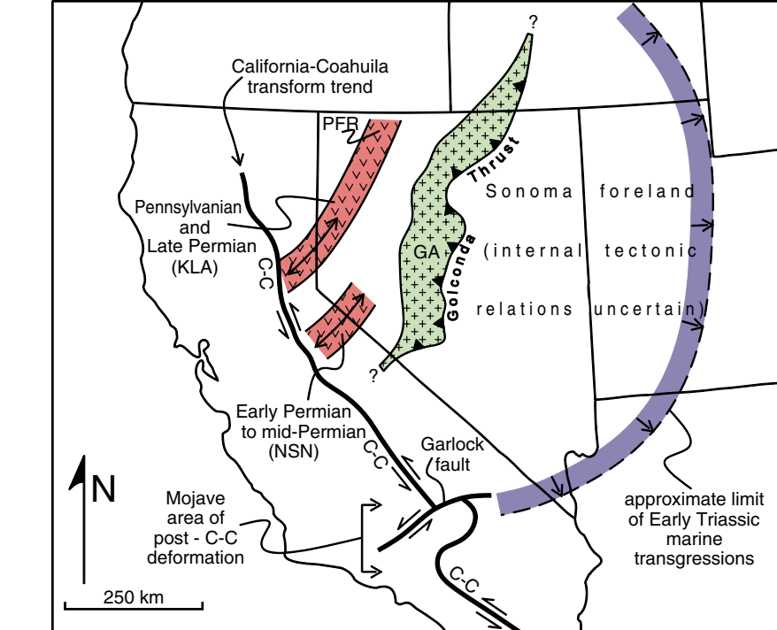
Figure 5. Syn-Sonoma (ca. 250 Ma) paleotectonic map of the Great Basin and adjacent areas (GA—Golconda allochthon) near the Permian-Triassic time boundary during oblique truncation of the Cordilleran continental margin by the California-Coahuila transform (C-C), which is contorted and offset by younger deformation in the Mojave region south of the Garlock fault. Eastern Klamath Mountains (KLA) and northern Sierra Nevada (NSN) arcs and remnant arcs (double-headed arrows denote NE-SW tectonic trends within the island-arc complex) are shifted SSE by 210 km to reverse Early Cretaceous dextral slip along the Mojave-Snow Lake fault, and the Klamath Mountains block is additionally shifted eastward to align with the Sierra Nevada block prior to Early Cretaceous forearc extension (Constenius et al., 2000) and later translation associated with Paleogene clockwise rotation of the Pacific Northwest (Oregon-Washington) Coast Range (see Fig. 8). PFR—Pine Forest Range.
